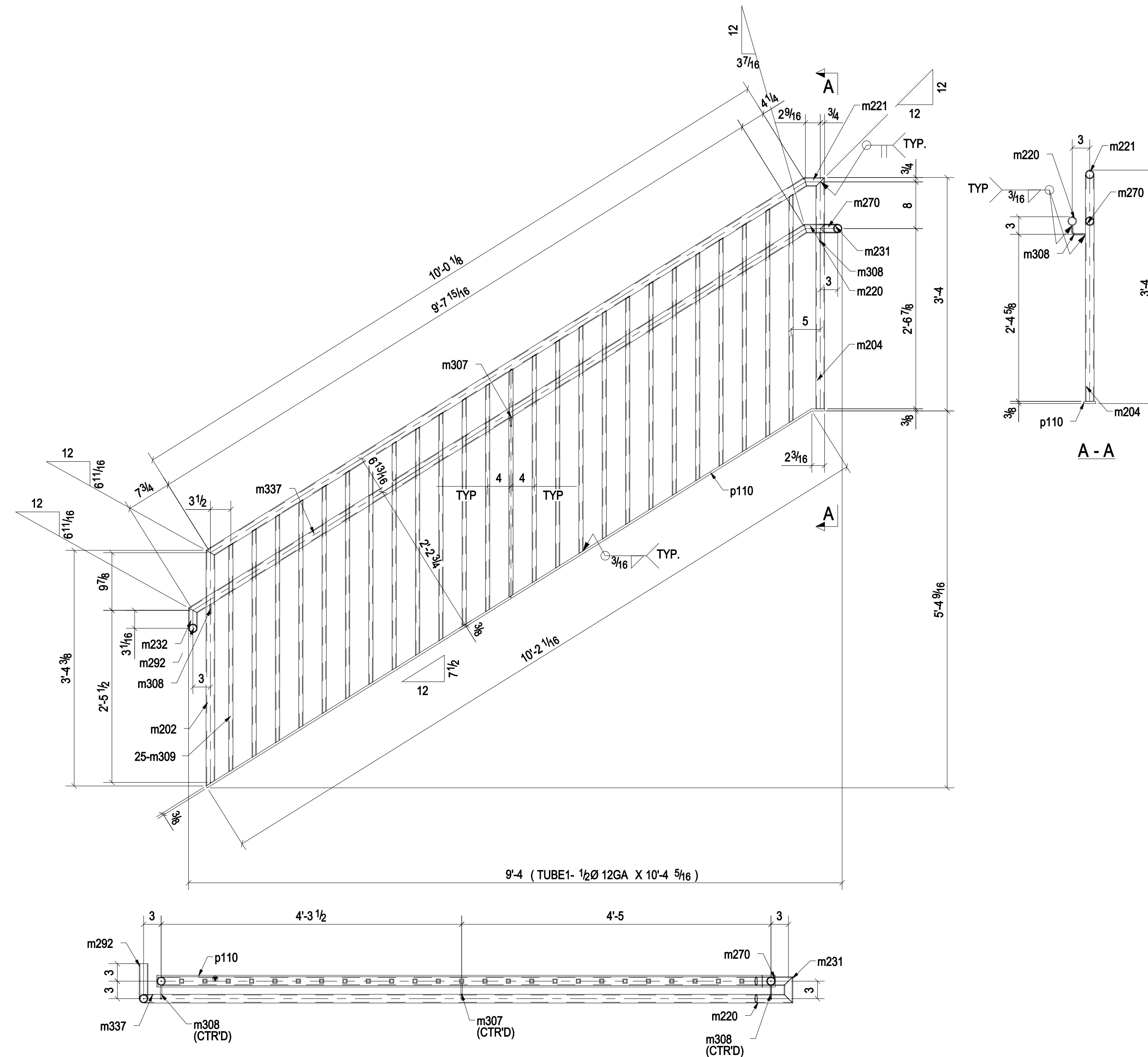
ONE - HANDRAIL - 133HR1
