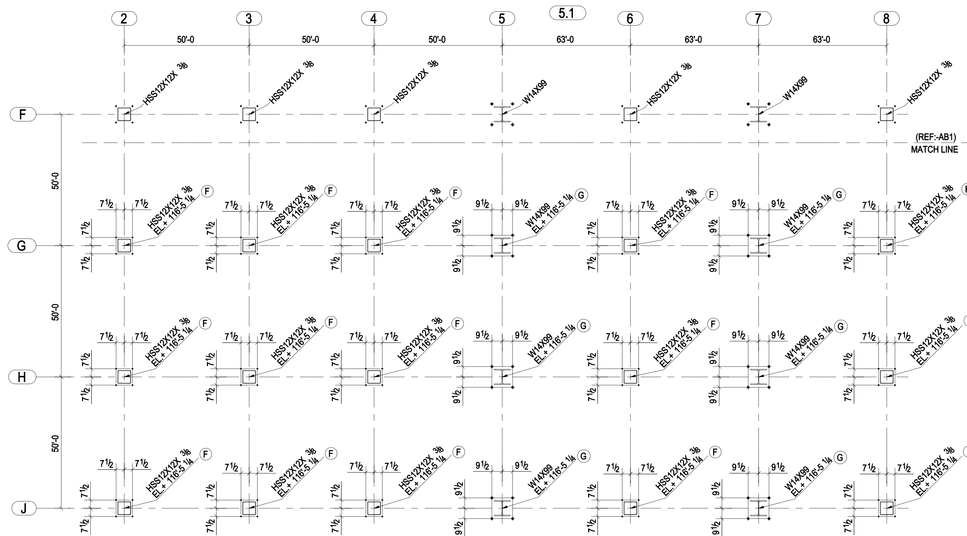
ANCHOR BOLT LAYOUT PLAN @ PART 'C' (REF-S101c)
