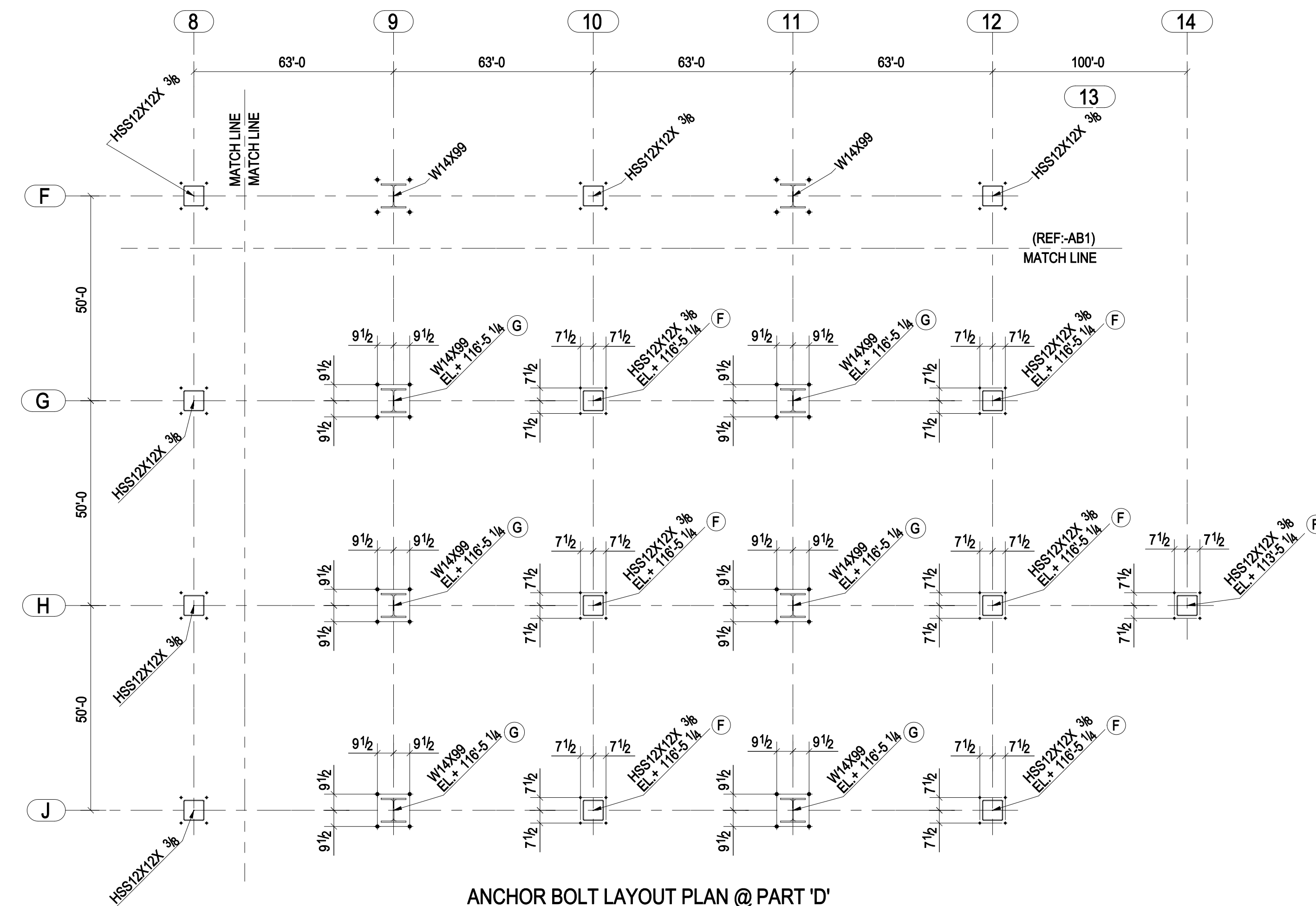
ANCHOR BOLT LAYOUT PLAN @ PART 'D' (REF-S101d)
