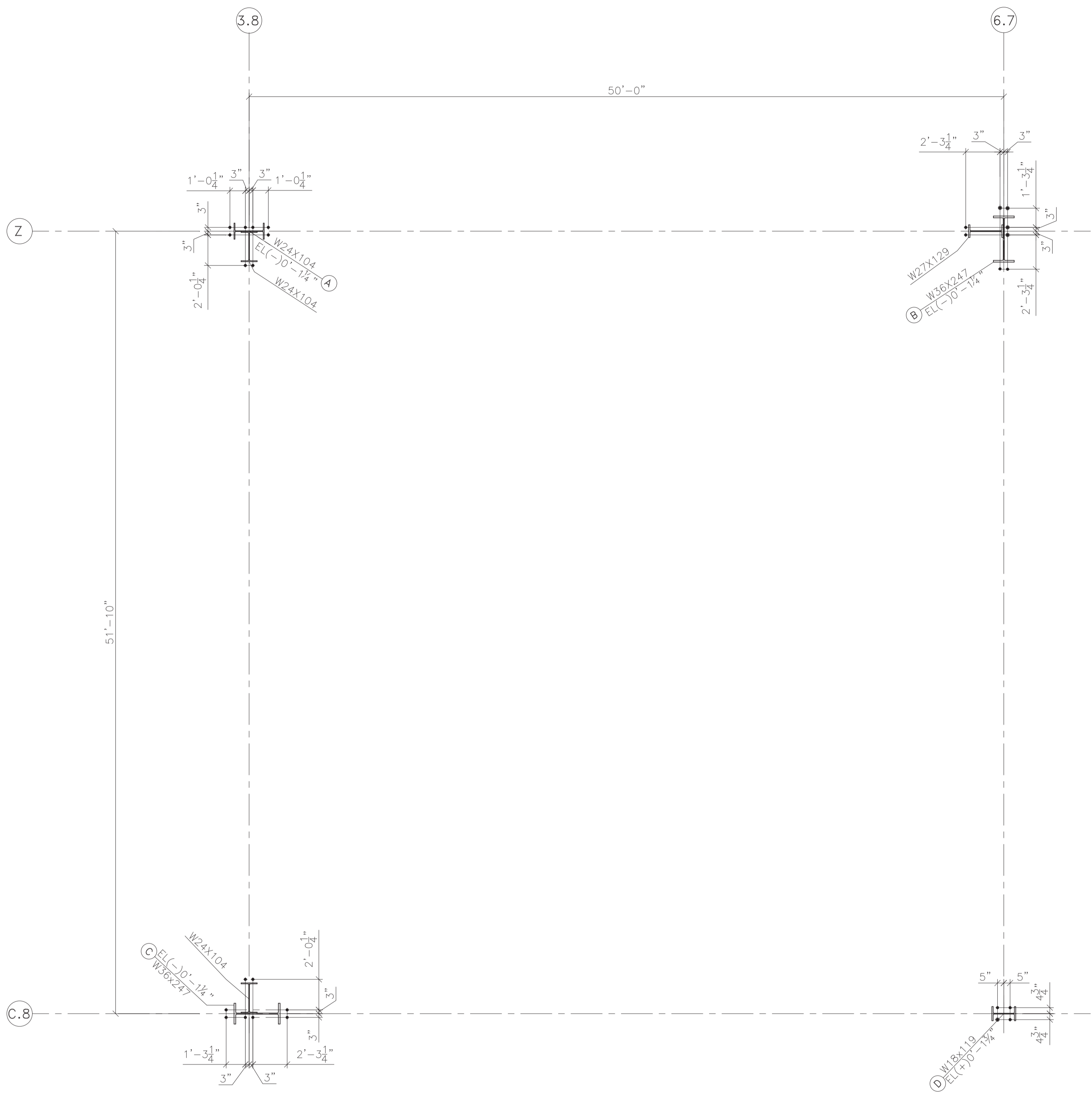
ANCHOR BOLT LAYOUT PLAN PLAN NORTH TRUE NORTH (REF: S101)
