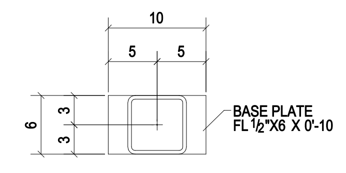
DETAIL-C (02 LOCATIONS)
