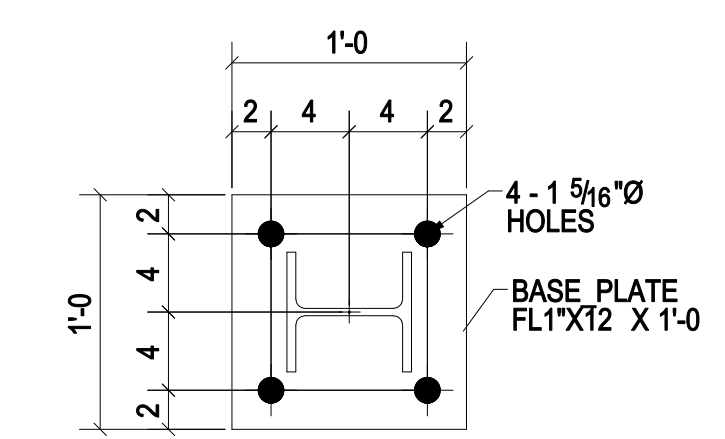
DETAIL-D (04 LOCATIONS)
