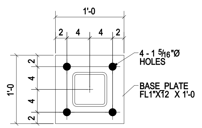
DETAIL-A (19 LOCATIONS)
