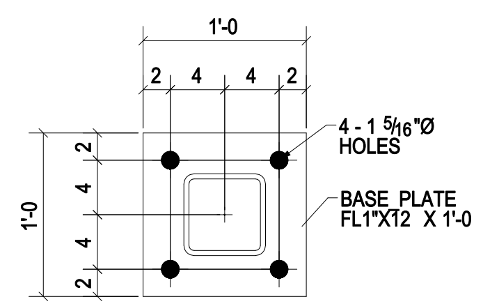
DETAIL-B (06 LOCATIONS)
