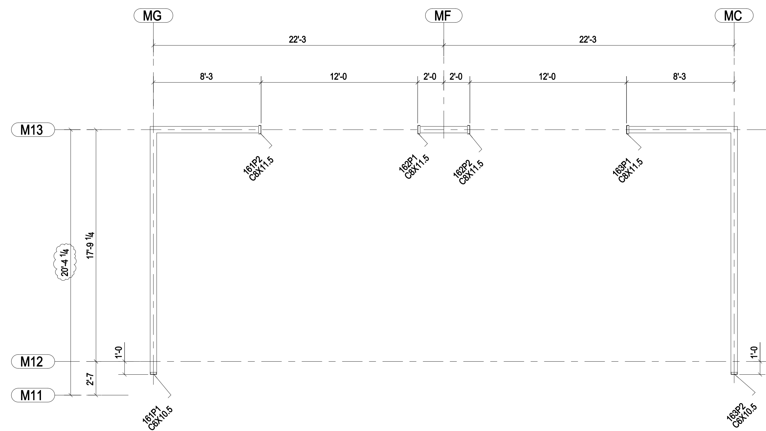
FLOOR FRAMING PLAN-LEVEL 1-SECTOR C & D (REF - S2.1B)
